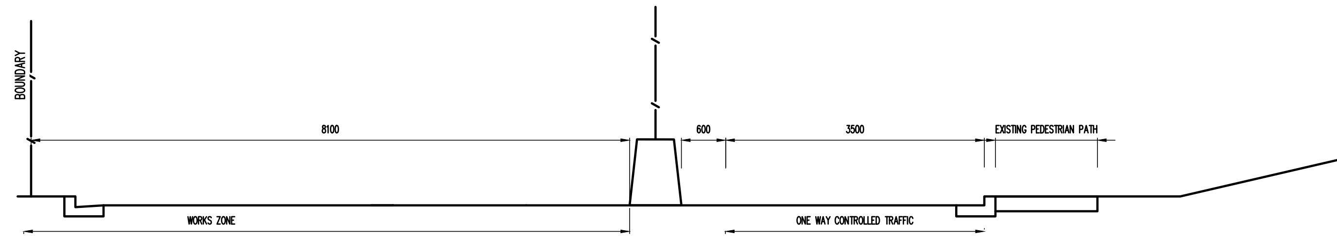
SECTION 1 SCALE 1:50
